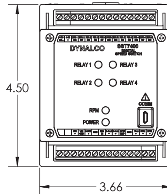
LED Model SST7200 / SST7400
