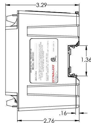
SST7200 / SST7400 / SST7200D / SST7400D
