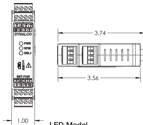
LED Model SST7000 / SST7100
