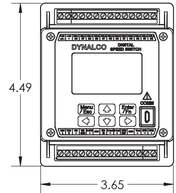
LCD Model SST7200D / SST7400D
